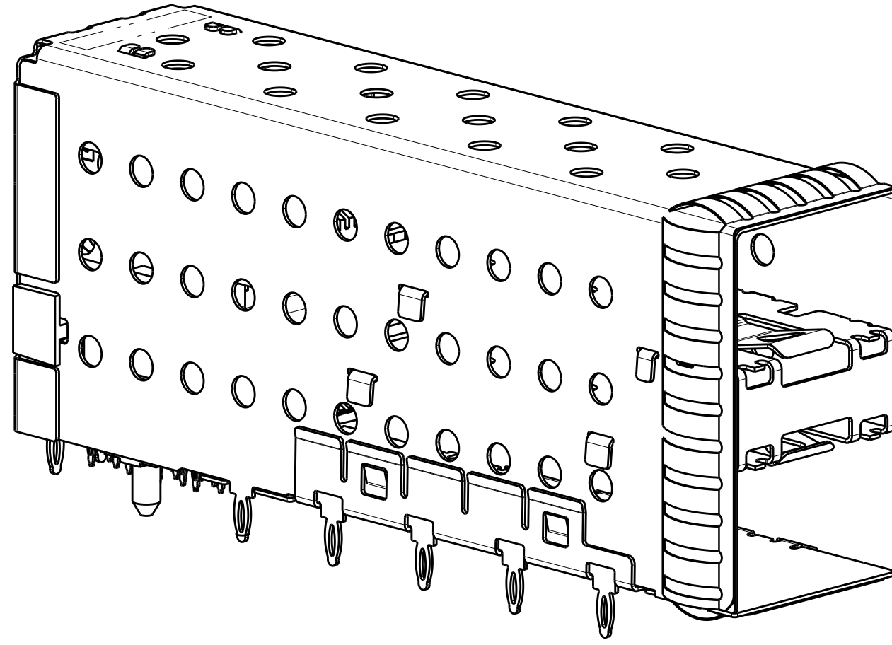
2007492-8, 1-2007492-8 AND 2-2007492-8 SCALE 3:1
