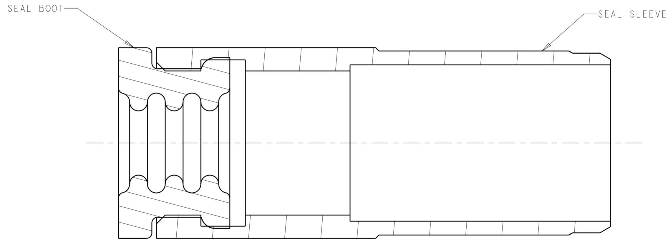
SECTION J-J
