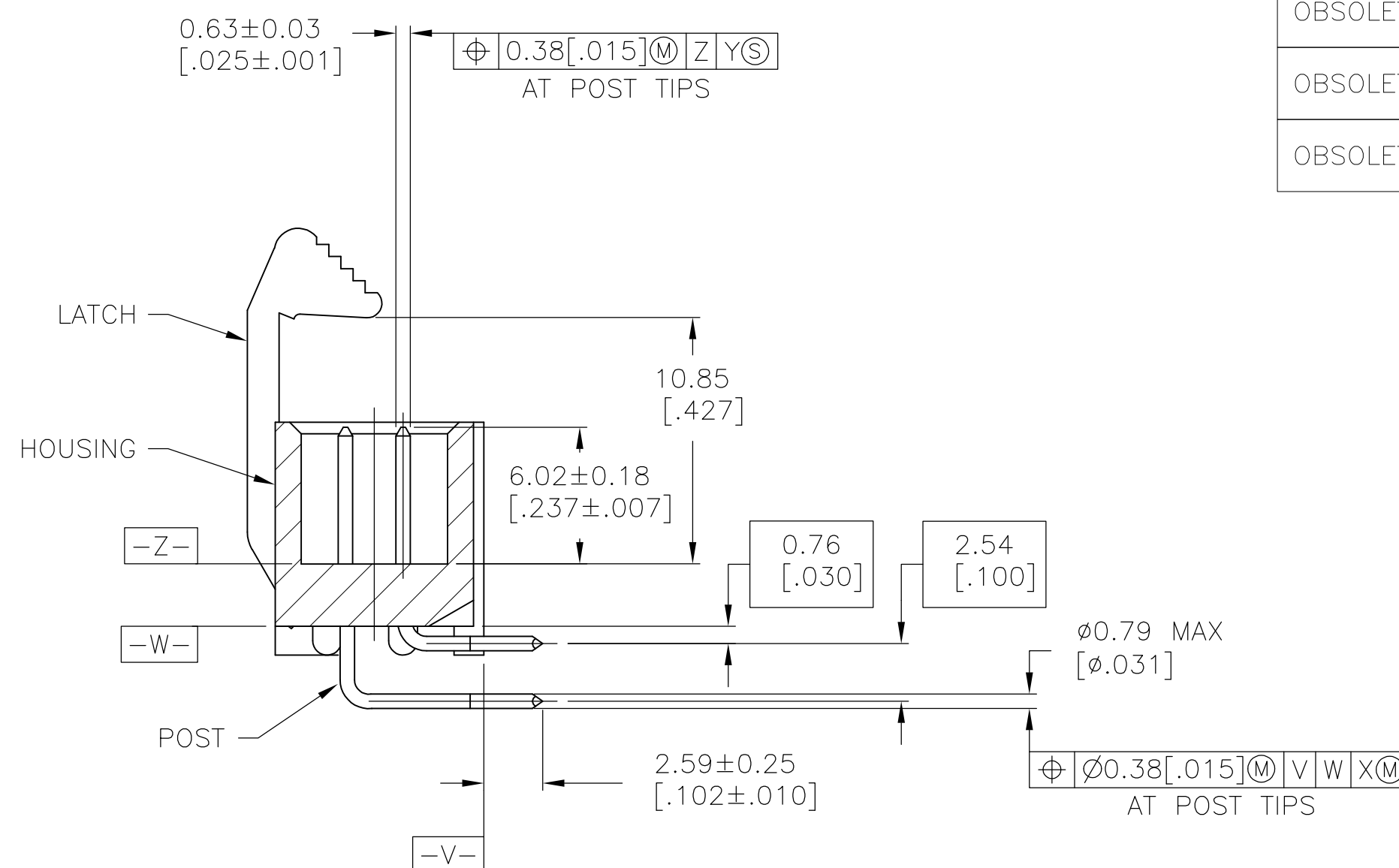
SECTION U-U
