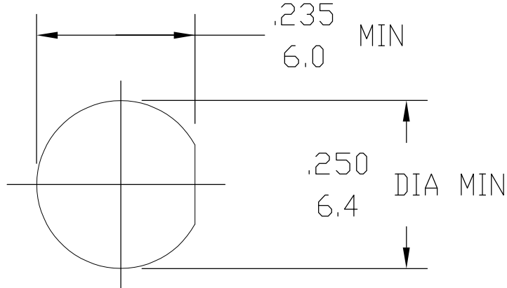
RECOMMENDED MOUNTING HOLE
