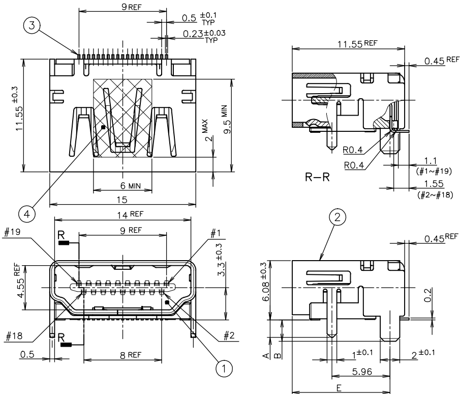
CONNECTOR WITHOUT FLANGE TYPE
