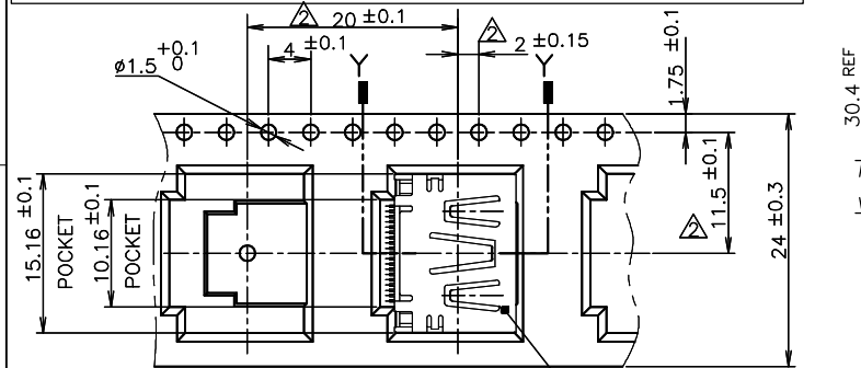
DETAIL X
