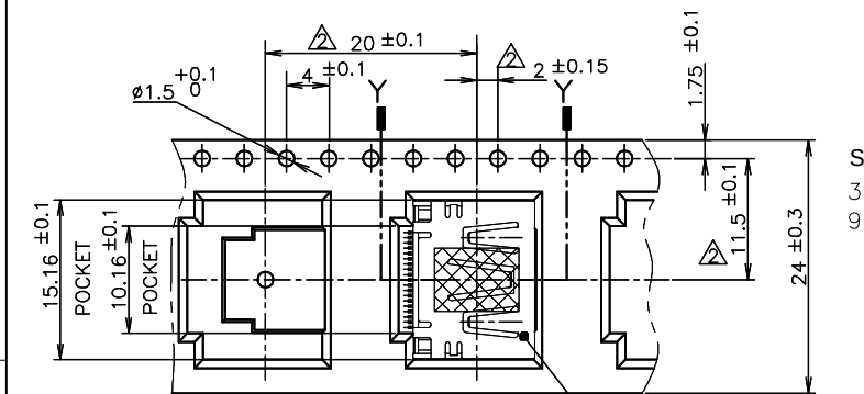
DETAIL X
