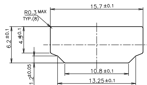
PANEL CUT OUT DIMENSION (REFERENCE)
