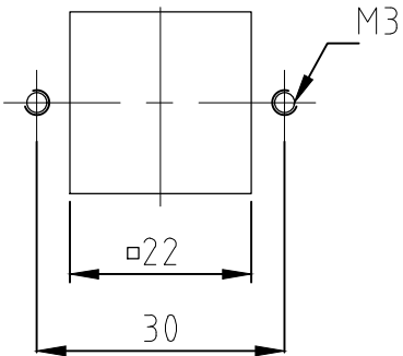
Panel cut-out for PN 0-4
