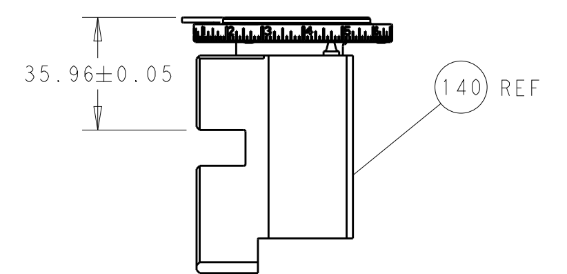
RAM SET-UP
