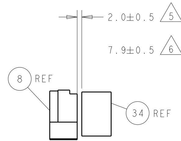
TERMINAL SUPPORT LOCATION
