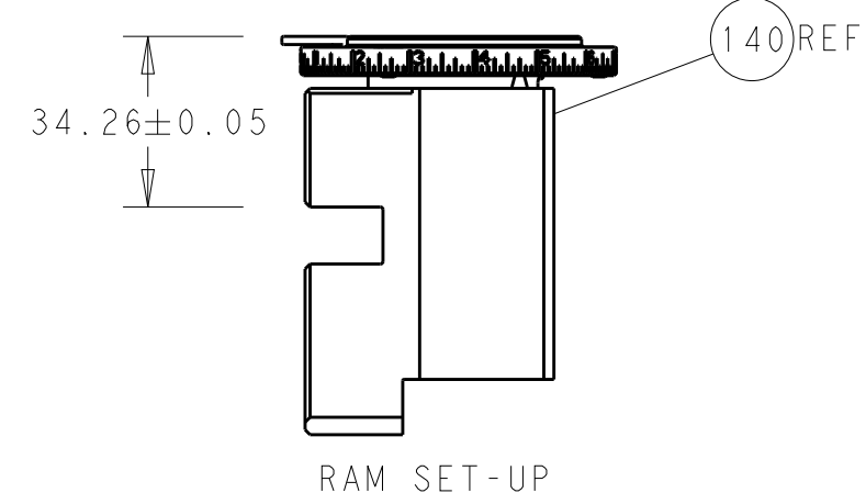
RAM SET-UP
