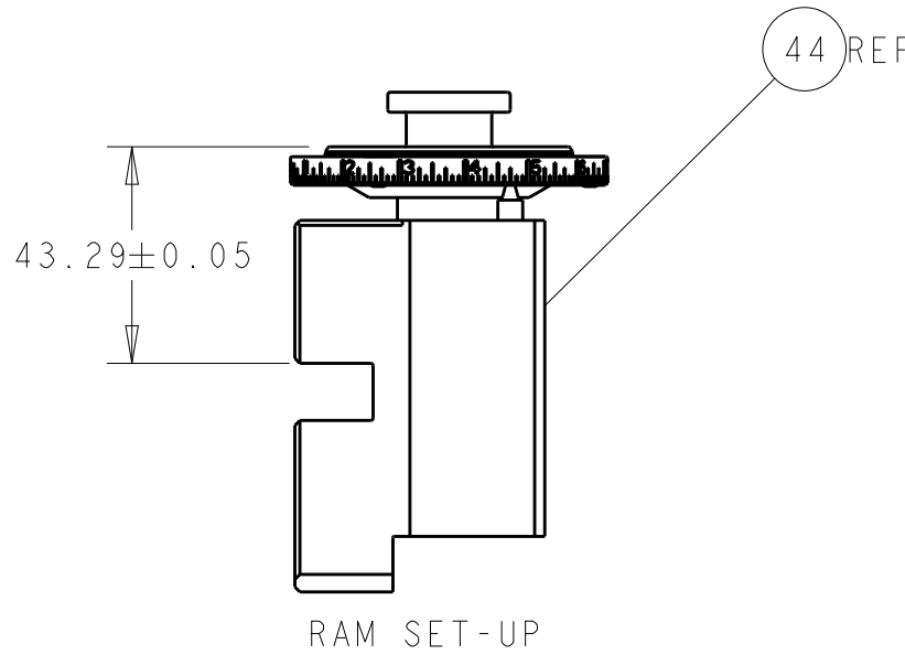
RAM SET-UP
