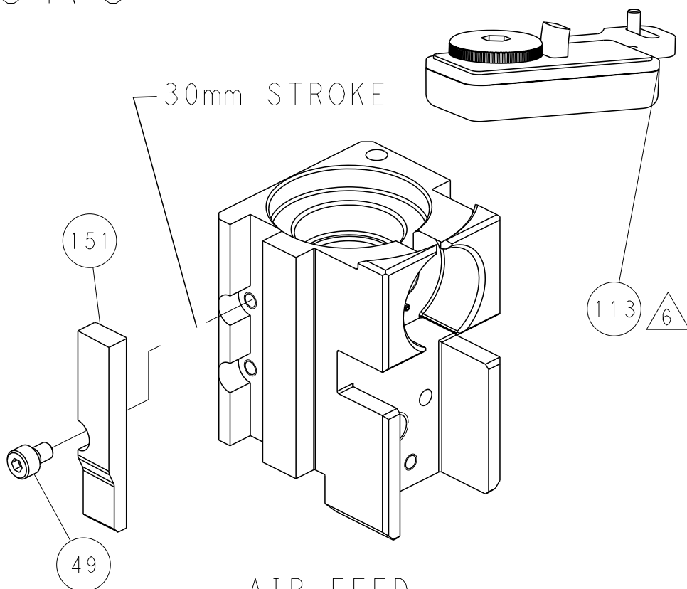
AIR FEED
