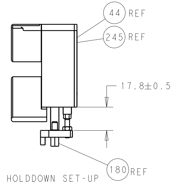
HOLDDOWN SET-UP
