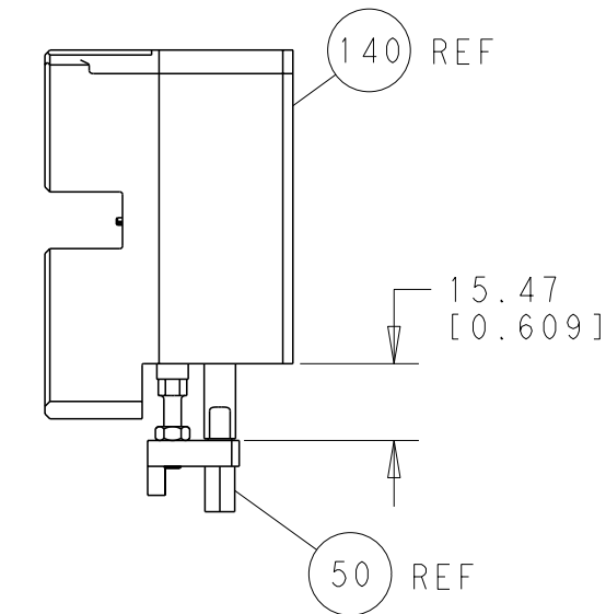
HOLDDOWN SET-UP
