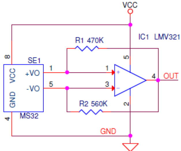
Figure 5: Switching point detection without hysteresis
