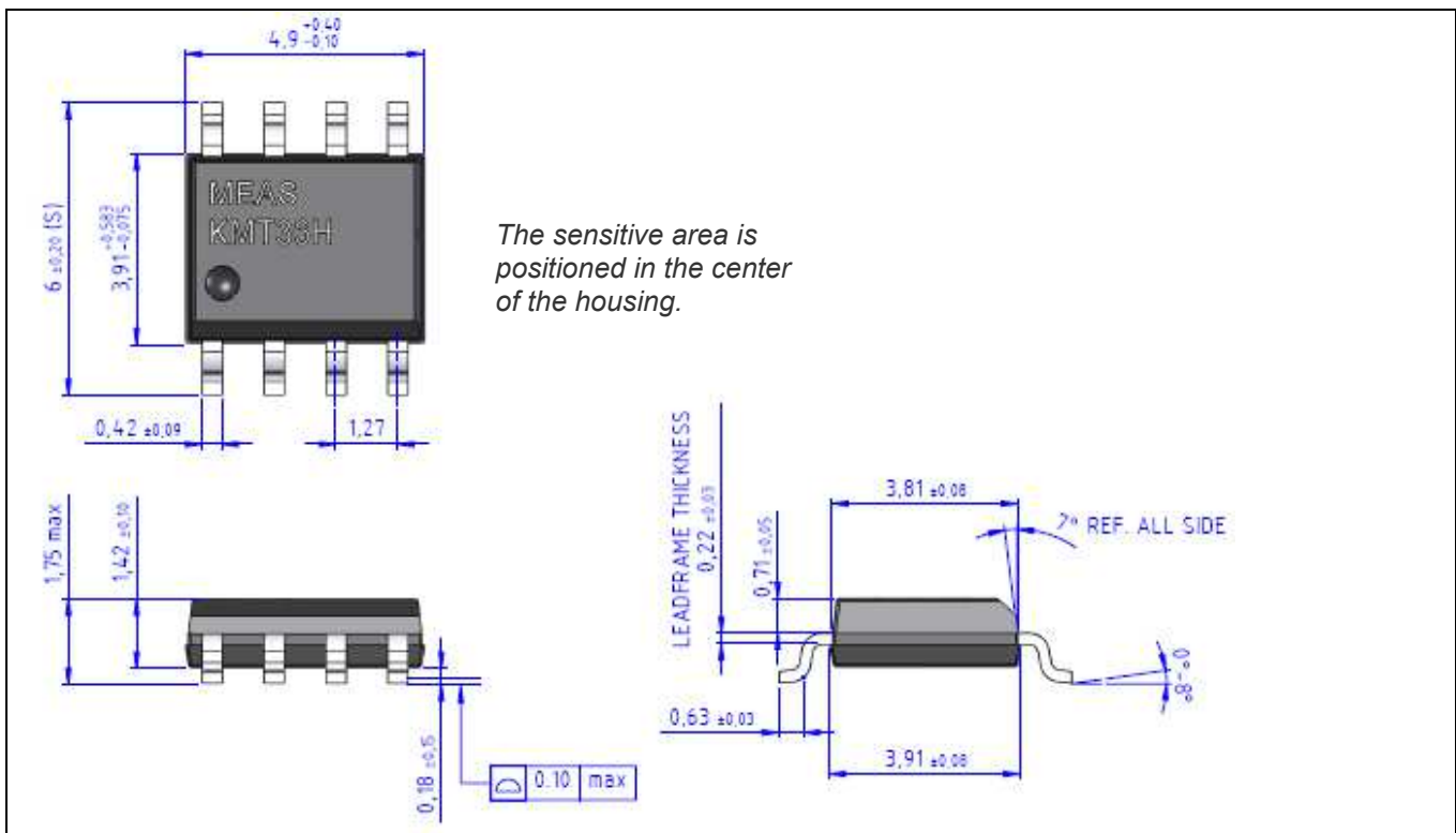
Figure 2: SO8 outline
