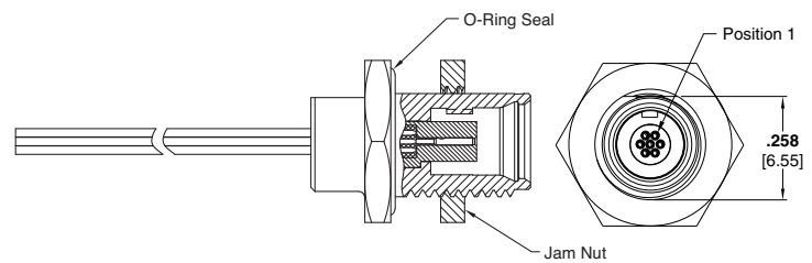
7 Position Drawing Number 1589060
