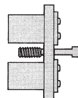
Modification 30 (RME, MME—threaded holes)
