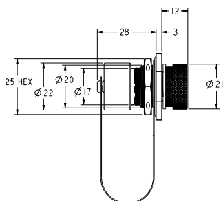
38999 Jam-Nut Receptacle Shell Kit for mini EB
