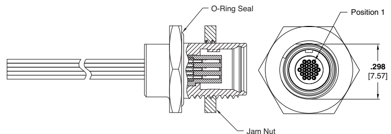
19 Position Drawing Number 1589061
