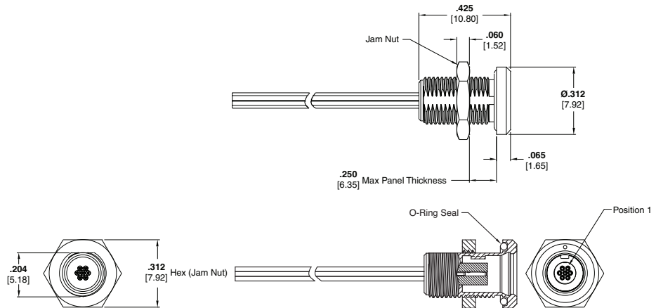
7 Position Drawing Number 1589056
