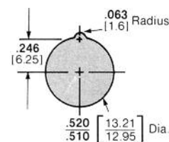
Recommended Panel Cutout for Bulkhead Mounting
