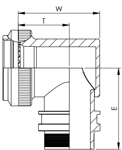
90° BACKSHELL - TYPE 1
