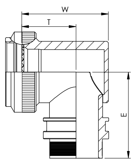
90° BACKSHELL - TYPE 1
