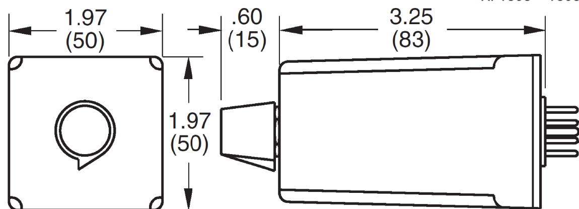
Outline Dimensions
