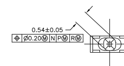
VIEW Z-Z SCALE 20:1
