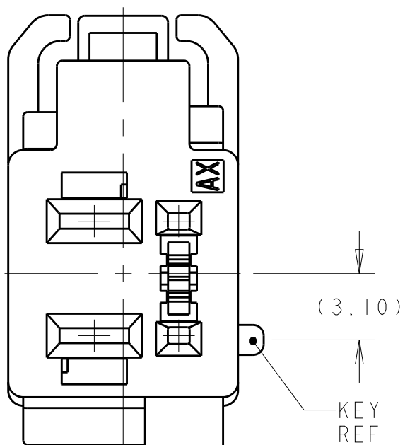
DETAIL E SCALE 4:1
