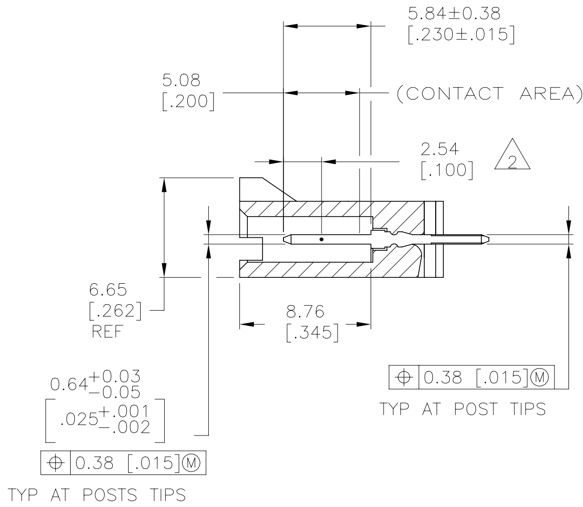
SECTION X-X
