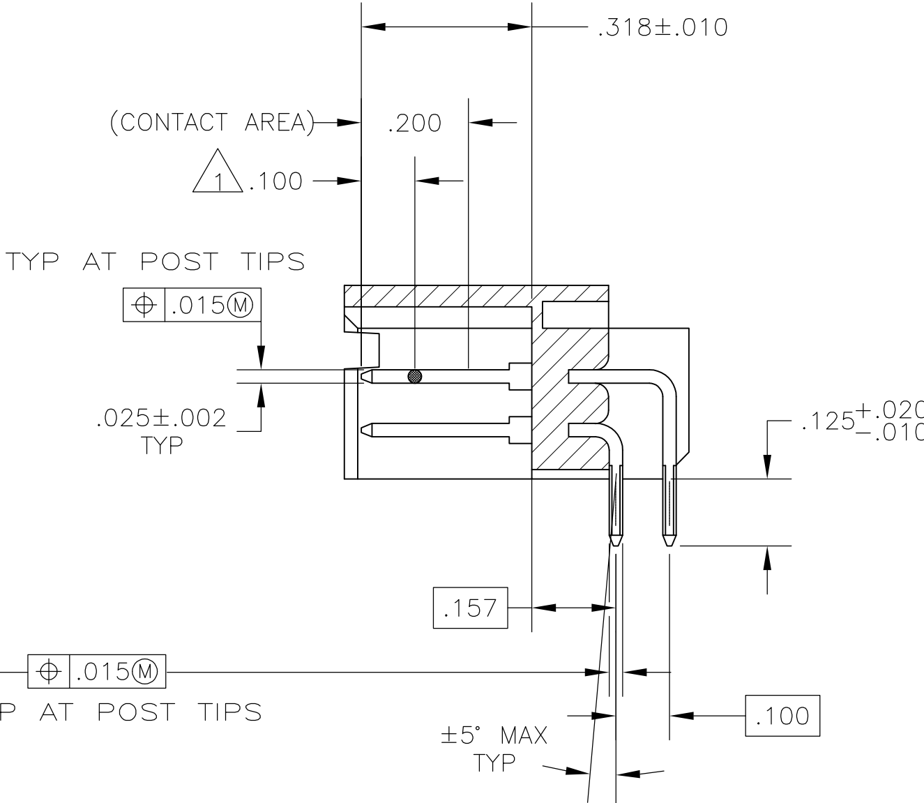
SECTION X-X
