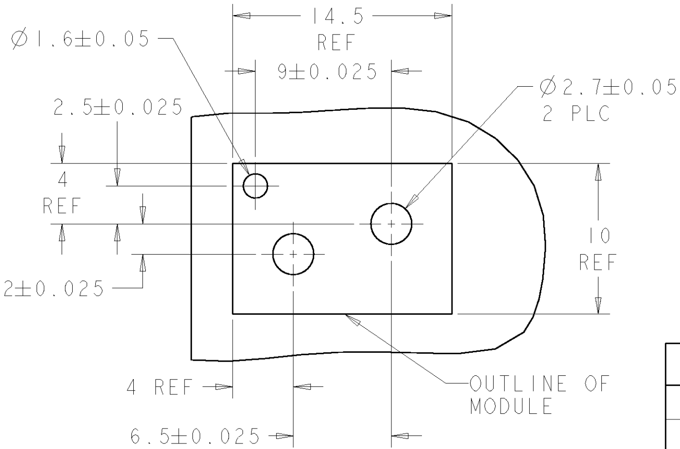
PCB LAYOUT
