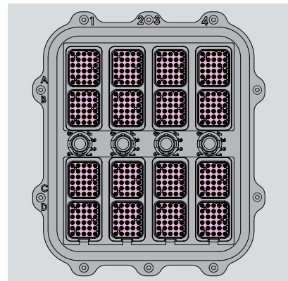
DMC-M Connectors Insert 30-23 Size 23 Contacts, 5A 480 contacts 175 g (without panel) 10 mounting screws 1 panel cutout
