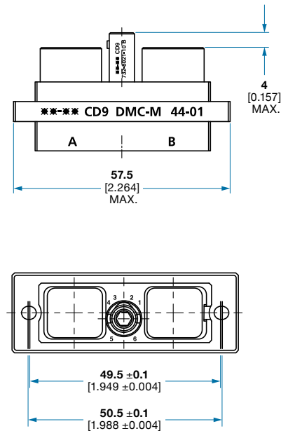
DMC-M 44-01: 2 Modules
