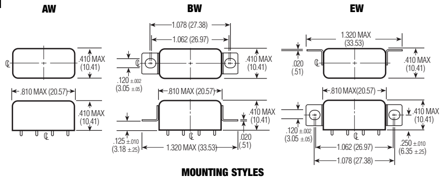
MOUNTING STYLES
