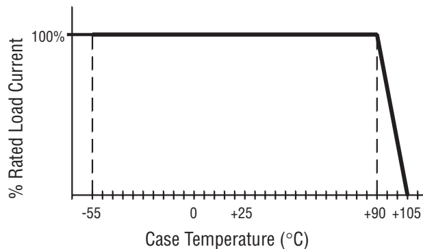
Figure 4 - Thermal Derating
