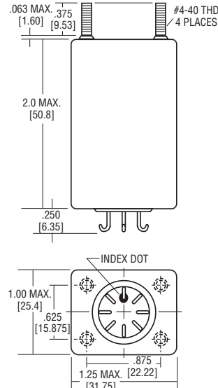
Mounting Option B
