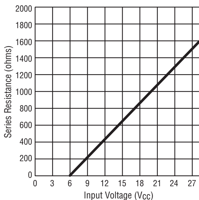
Figure 2 - Series Resistance vs. Vcc Input Voltage (Note 1)
