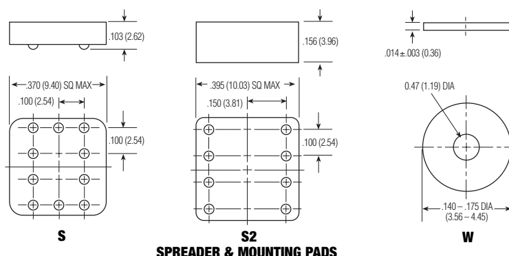
SPREADER &amp; MOUNTING PADS
