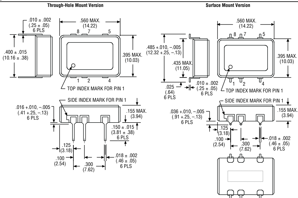
Figure 7 - Outline Dimensions
