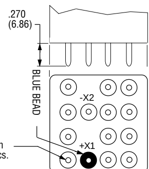
CODE "G" Circuit Board Pins- 28 VAC Coils
