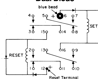
CODE 6 Dual Diode
