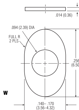
MGST MOUNTING PAD
