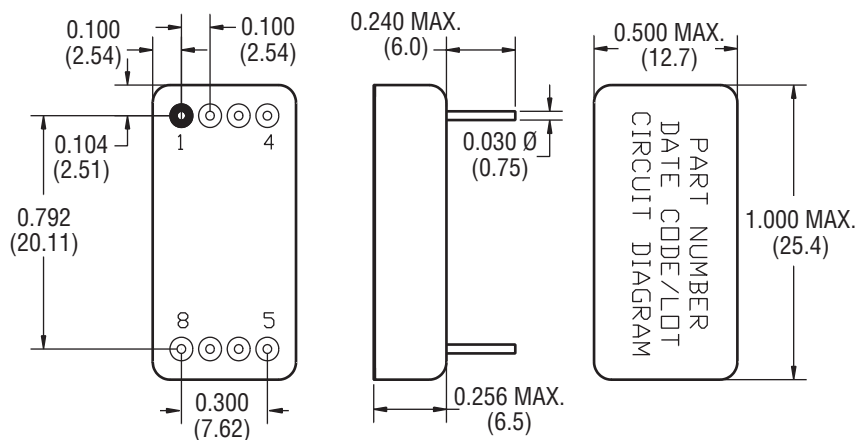
Figure 6 - Outline Dimensions
