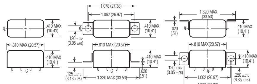
MOUNTING STYLES
