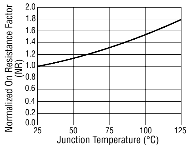
Figure 6 - On-Resistance vs. Temperature (Note 6)
