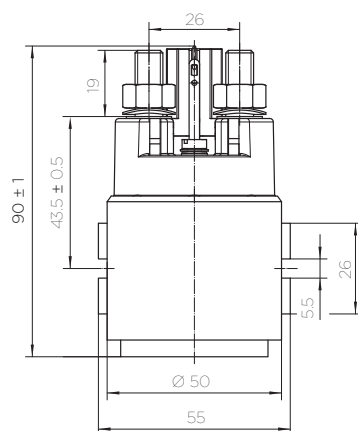
Short form side mounting
