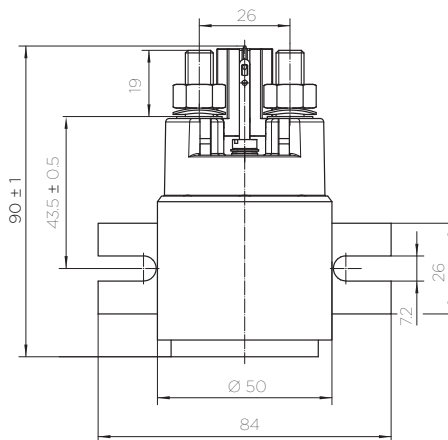
Long form side mounting
