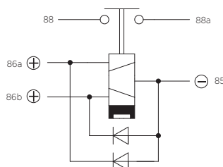
Suppression diode 30-100-50
