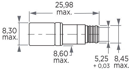
Female Contact
