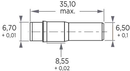
Sealing plug
