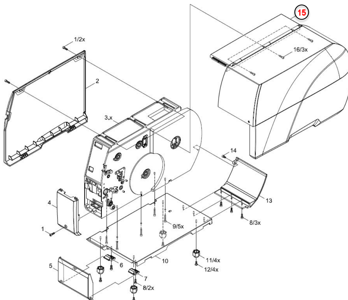
Figure 3 - T3212/T3224-PRINTER (cover)
