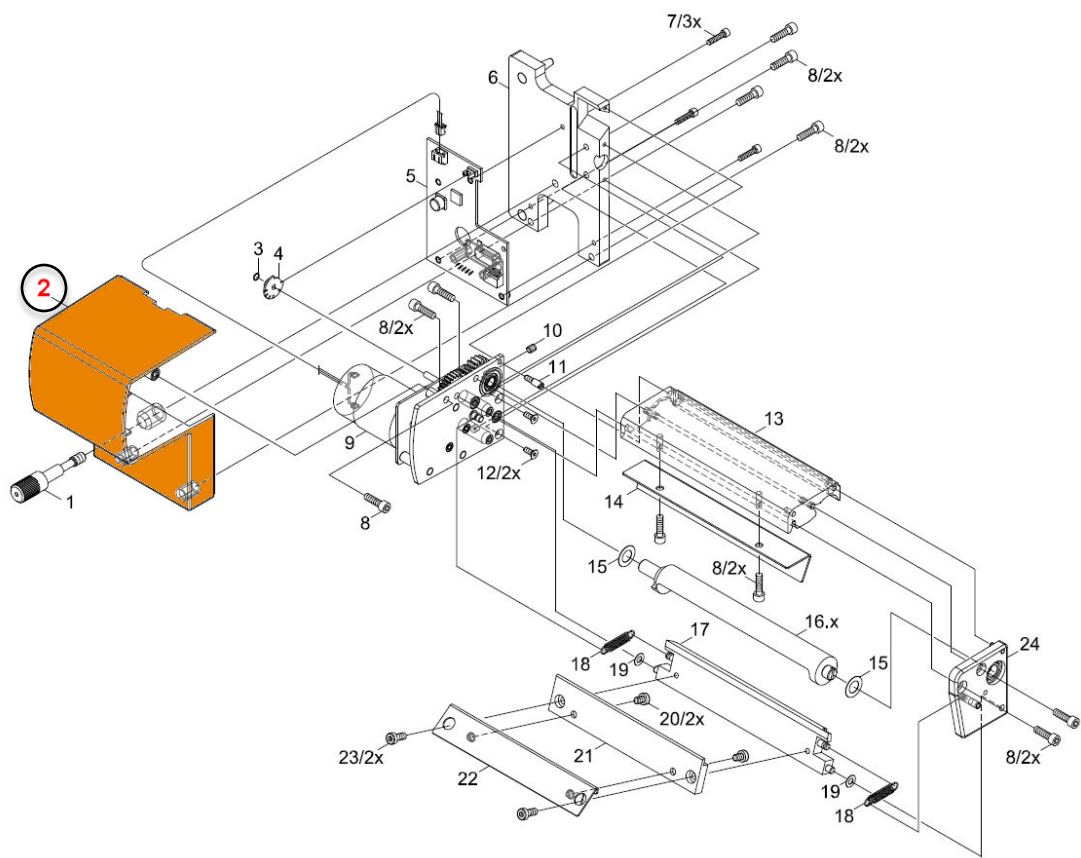
Figure 8 – T3212/T3224-PRINTER-CUTTER/PERFORTOR
