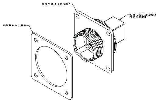
Receptacle Kit, Pass-through RJ45/RJ45 – Part No. 1776186-1
