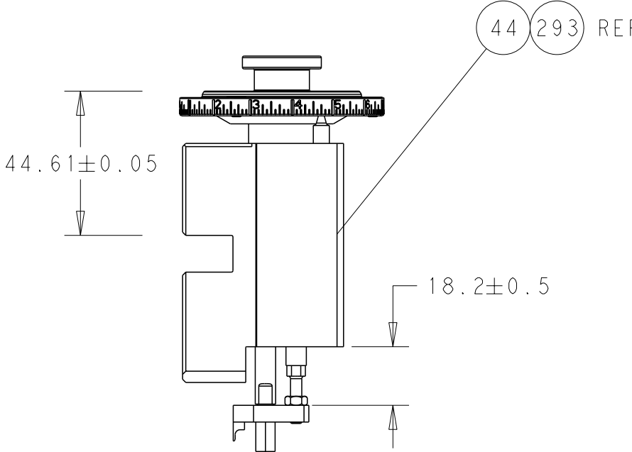
RAM SET-UP
