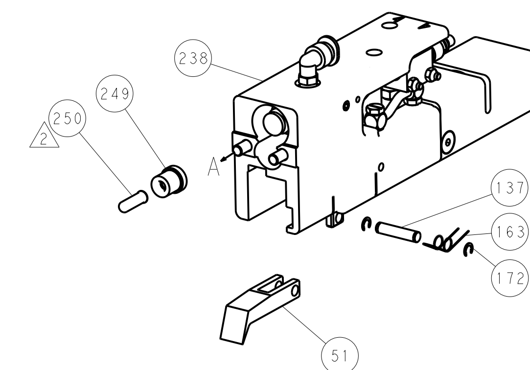
PNEUMATIC
