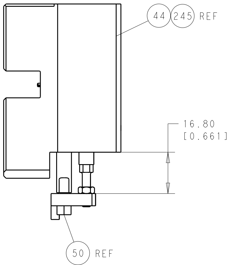
HOLDDOWN SET-UP
