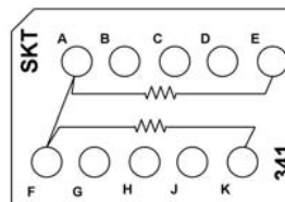
CTJ420E341 Two 470 k \Omega Resistors, 2 W
