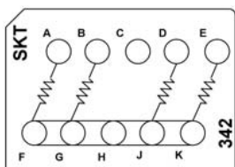
CTJ420E342 Four 1.5 k \Omega Resistors, 1 W
