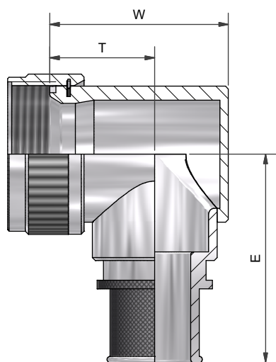
90° BACKSHELL - TYPE 1
