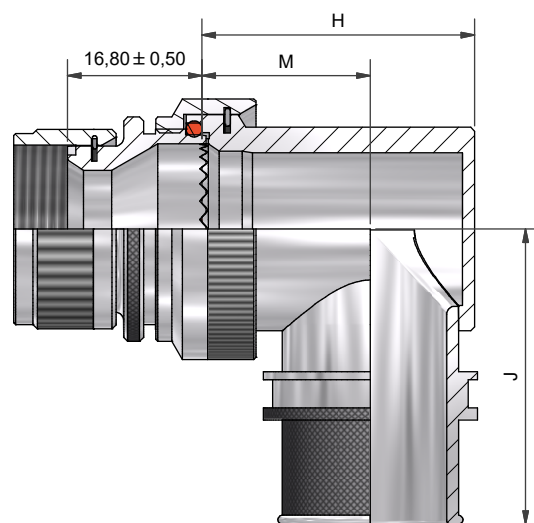
90° BACKSHELL - TYPE 2
