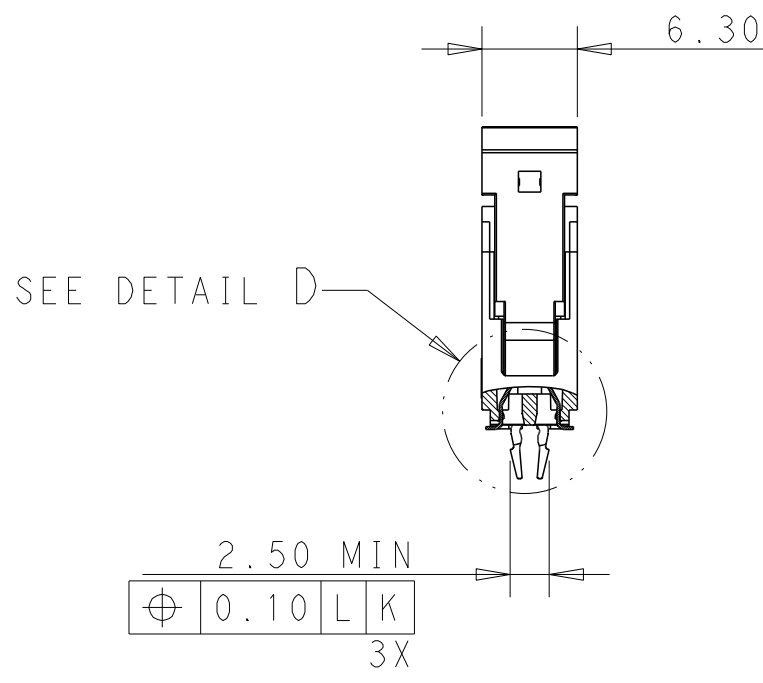
SECTION E-E
