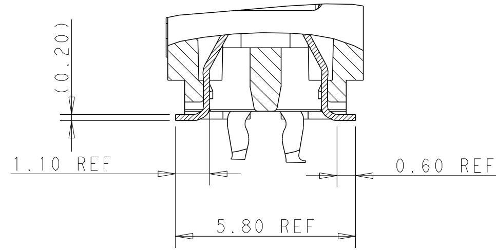
DETAIL D SCALE 8:1
