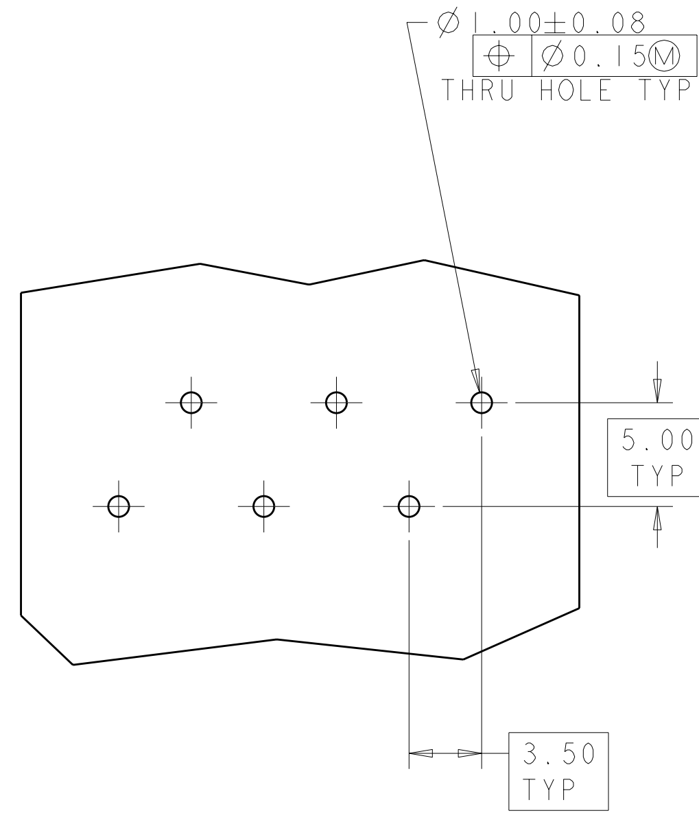
△ PCB FOOTPRINT SCHEME A SCALE 4:1
