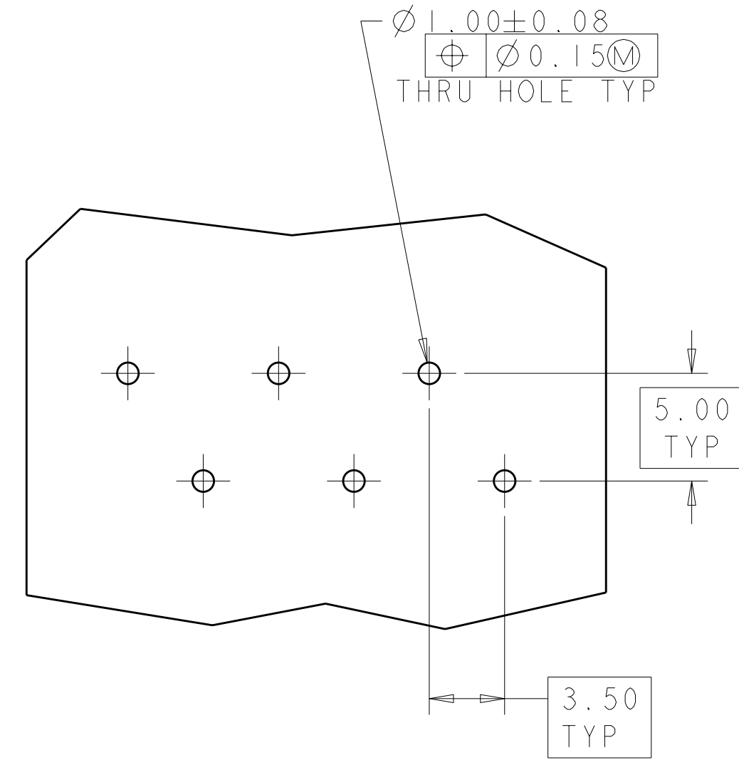
△ PCB FOOTPRINT SCHEME B SCALE 4:1
