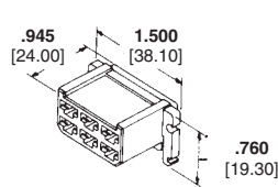
Receptacle Housing
