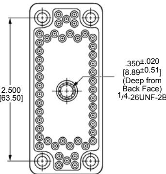
Receptacle Housing
