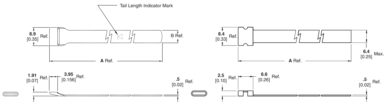
One Step Clamping Band — Straight
