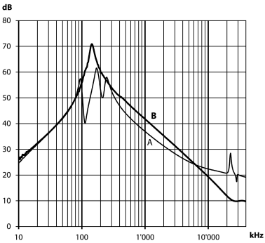
250/400/600 A types
