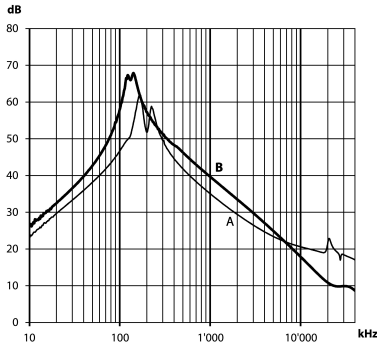
1000 A types
