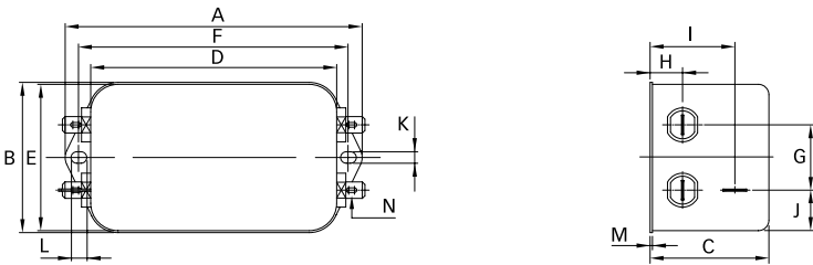
Connection style -06, 6 to 12 A types
