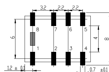
SMT Gull wings version
