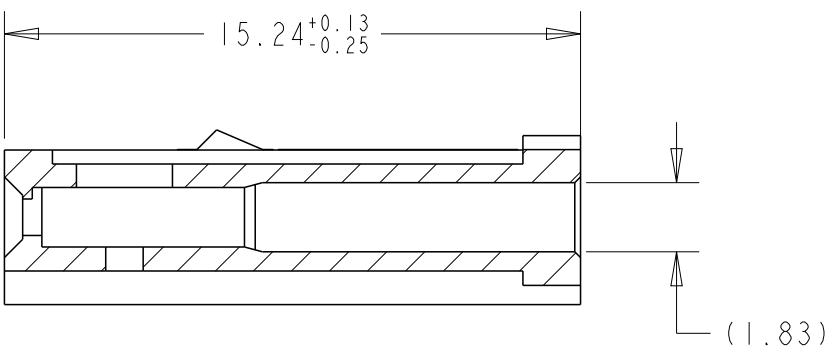
SECTION X-X
