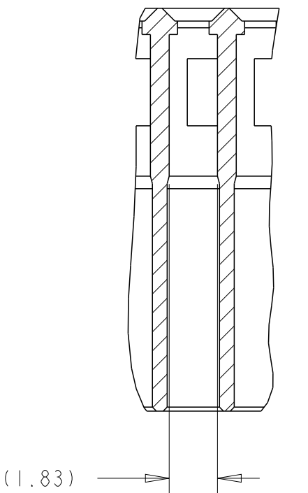
SECTION Y-Y
