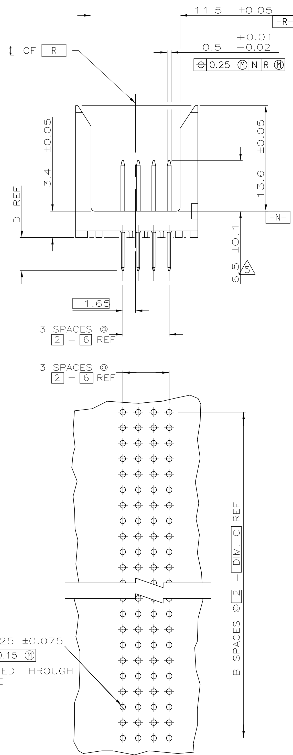
RECOMMENDED CIRCUIT PATTERN PER IPC-D300 TYPE II, CLASS C (COMPONENT SIDE)
