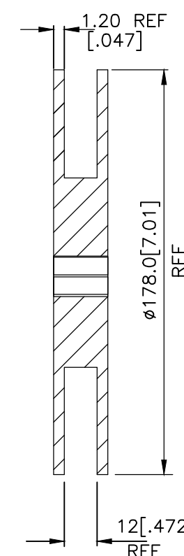
Section C—C
