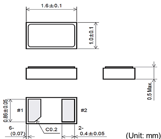
Top View Crystal Connection
