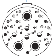
2520 Service N 10 Contacts, Size 20 13 Contacts, Size 16 4 Coax Contacts, Size 12 3 Twinax Contacts, Size 8
