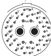
2546 Service I 40 Contacts, Size 20 4 Contacts, Size 16 2 Coax Contacts, Size 8
