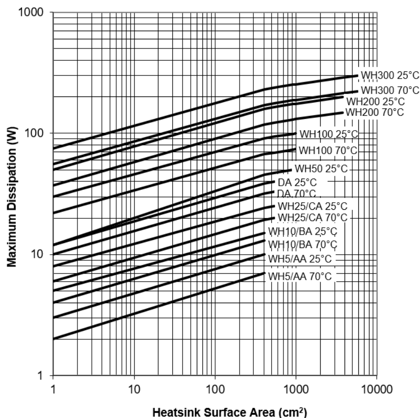
Derating for Reduced Heatsink Dimensions
